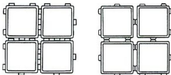
ABOVE LEFT Rima should be installed with spacers intertwined with the neighbouring block for water drainage ABOVE RIGHT Rima should be installed with spacers touching to achieve larger joints for joint growth
