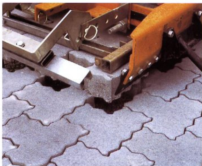
ABOVE Mechanised laying of the new Matoro Block
